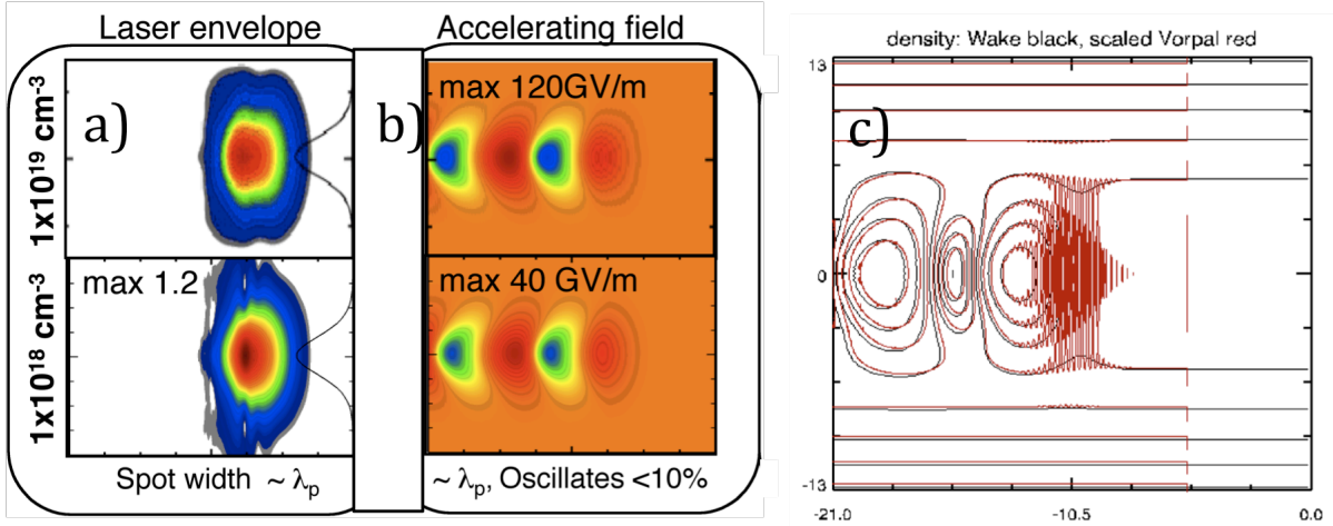
FIGURE 1. Scaled simulations of a mildly nonlinear 10 GeV stage using 40 J energy at n=10^{17} \text{ cm}^{-3} . (a) Laser envelope for 10^{19} \text{ cm}^{-3} (top) and 10^{18} \text{ cm}^{-3} (bottom), (b) accelerating field structure for 10^{19} \text{ cm}^{-3} (top) and 10^{18} \text{ cm}^{-3} (bottom). The wake amplitude, dephasing and depletion distances as well as energy gain scale with density as predicted. (c) Plasma density n/n_0 contours on a fixed scale for (black) WAKE 3D axisymmetric quasistatic PIC simulations at 10^{17} \text{ cm}^{-3} density and (red) VORPAL 2D slab scaled simulations at 10^{19} \text{ cm}^{-3} . The results are nearly indistinguishable from each other except for the fast laser oscillations not modeled in WAKE.
